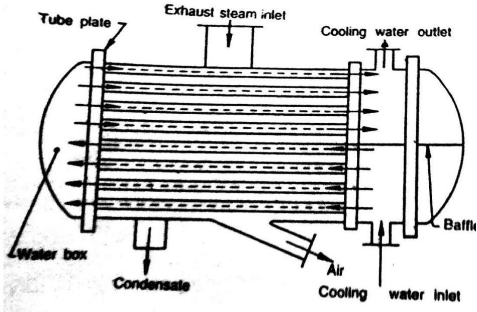
Fig. 6.5 Surface Condensers
