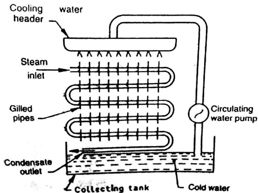
Fig. 6.8 Evaporative Condenser
