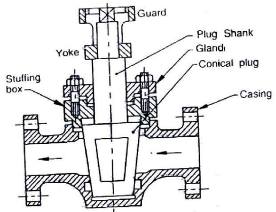
Fig. 3.10 Blow off cock
